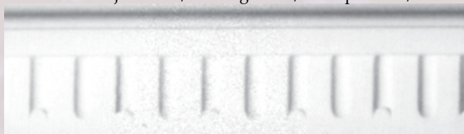
FM348 Projection: 7/8" Height: 2 1/4" Repeat: 1 3/8"
