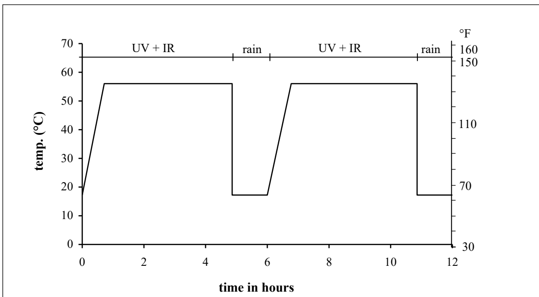
Figure 2.4.1. Cycles weather-o-meter.
